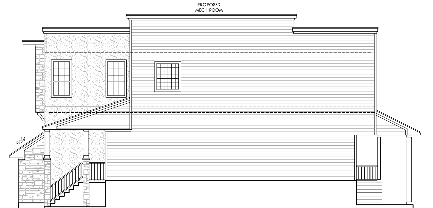
REAR ELEVATION 12'
