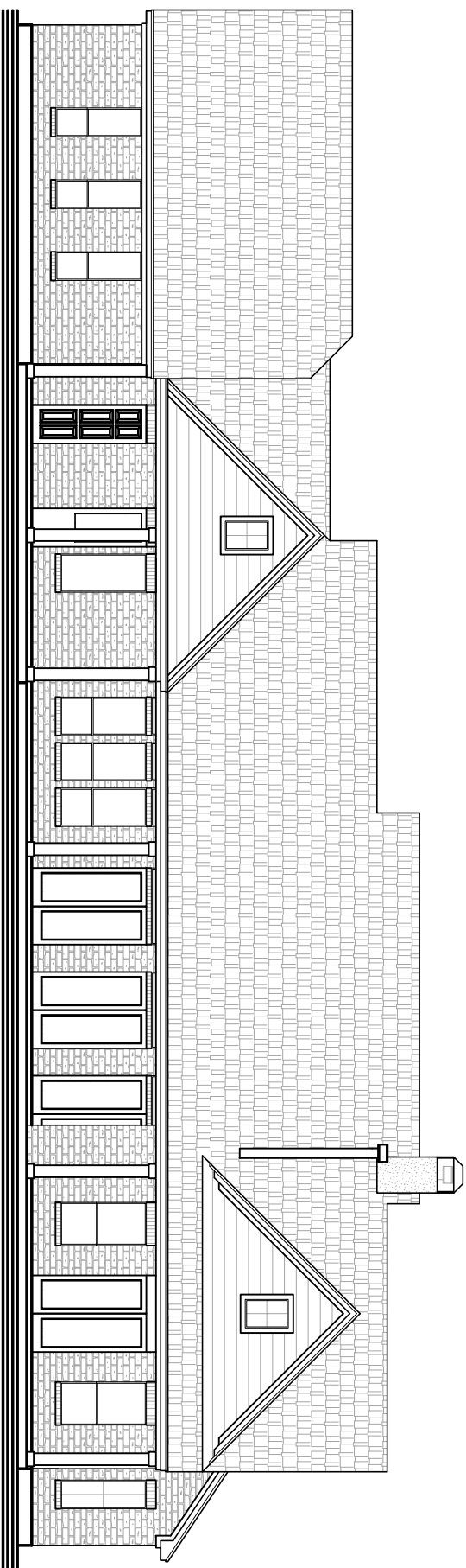
REAR ELEVATION
