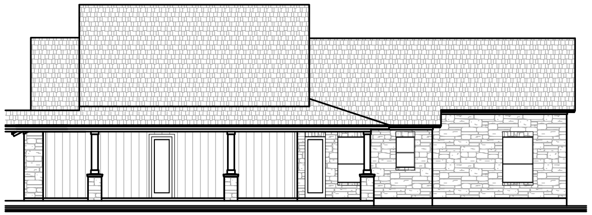
GARAGE REAR ELEVATION
