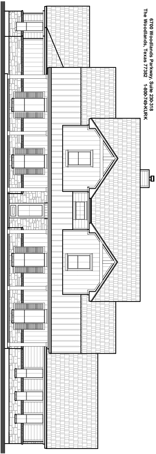
FRONT ELEVATION
