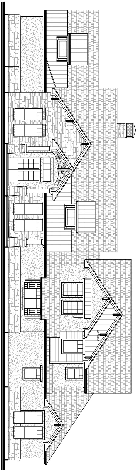
FRONT ELEVATION
